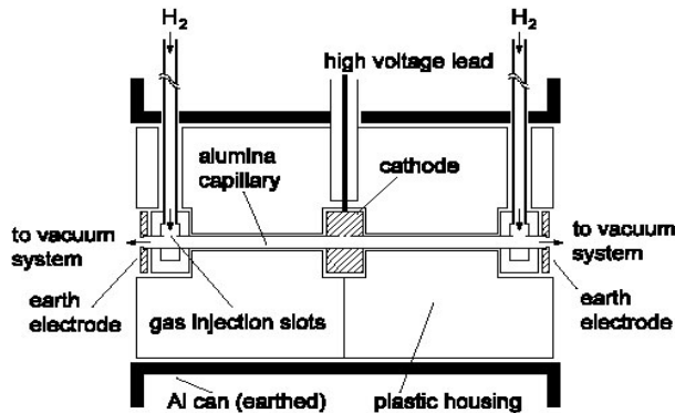
FIGURE 4. Schematic diagram of the H 2 -filled capillary discharge waveguide.
