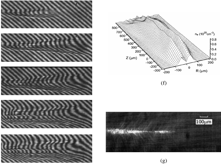
FIGURE 6. Interferograms of a plasma in the regime of relativistic self-focusing: (a) 0 ps, (b) 5 ps, (c) 15 ps, (d) 35 ps, and (e) 45 ps after the passage of a 4.3 TW laser pulse through a He gas jet with an atomic density of 4 \times 10^{19} \text{ cm}^{-3} . In (f) is shown the reconstructed electron density profile of the channel formed 35 ps after the passage of the pulse. An image of the Thomson scattered radiation from the passage of the driving laser pulse through the He gas jet is shown in (g). (From Sarkisov et al. [29])
