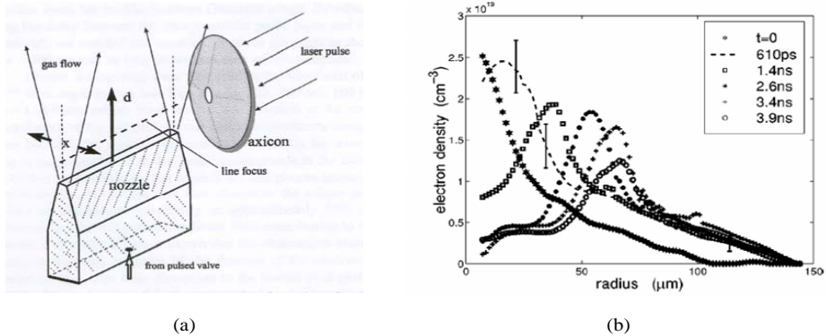
FIGURE 2. (a) Arrangement for forming a plasma channel by hydrodynamic expansion, and (b) the measured temporal evolution of the transverse electron density profile after the formation of a cylindrical plasma column in Ar at t=0 . (From Fan et al. [17] and Nitikin et al. [13]).
