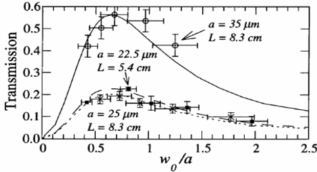
FIGURE 1. Measured and theoretical pulse energy transmission as a function of the ratio of the spot size of the input pulse, w_0 , to the capillary radius, a , for capillaries of three different radii. (From Dorchie et al. [5]).
