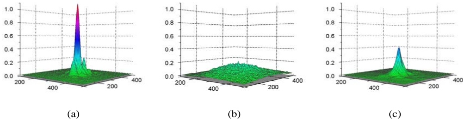
FIGURE 5. Measured transverse intensity profiles at the entrance and exit of a 30 mm long capillary discharge waveguide initially filled with 330 mbar of \text{H}_2 . Profiles are shown: (a) at the entrance to the capillary; and at the exit for pulses injected (b) prior to the onset of the discharge; (c) 731 ns after the onset of the discharge. The vertical and horizontal scales are in units of 10^{17} \text{ W cm}^{-2} and \mu\text{m} respectively.
