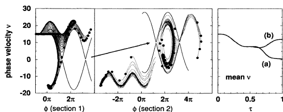
FIG. 2. Phase-space diagrams of electrons at saturation showing detrapping of lower energy electrons and capture of high energy electrons for \Delta K \approx 0.033 . Solid lines represent the separatrix in each undulator section. The solid dots represent the electrons at the end of each section. The right-hand side shows the mean electron energy down the undulator ( \tau = 0 \rightarrow 1 ) for \Delta K \approx 0.033 (a) and \Delta K = 0 (b). Step in K occurs at \tau = 0.5 .
