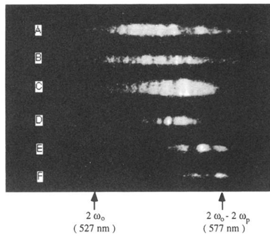
FIG. 1. Variation of second harmonic at 45° backscattered direction with respect to incident laser intensity: (a) 2.0 \times 10^{18} , (b) 1.5 \times 10^{18} , (c) 1.0 \times 10^{18} , (d) 6 \times 10^{17} , (e) 5 \times 10^{17} , and (f) 3 \times 10^{17} W/cm 2 .
