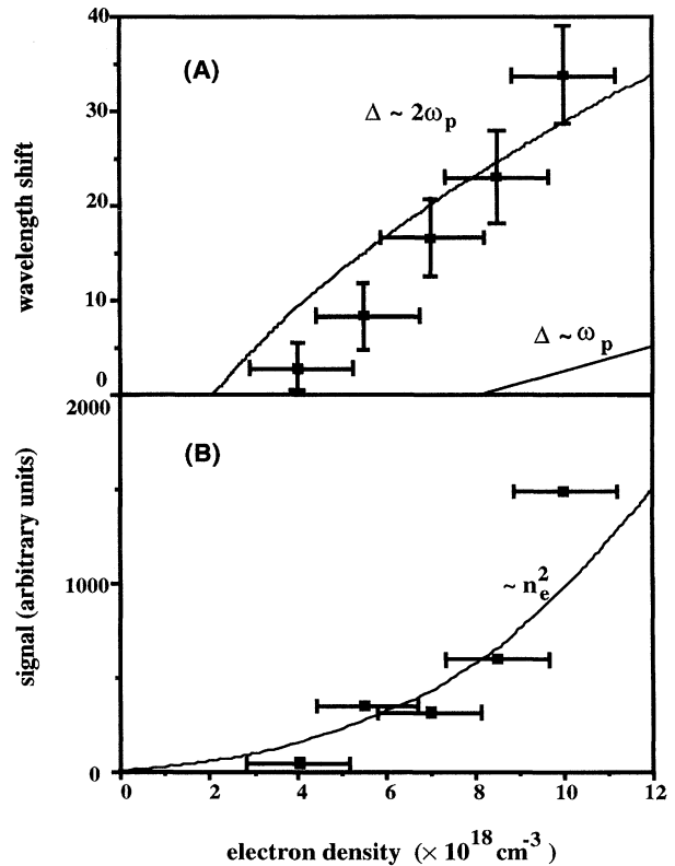
FIG. 2. (a) Wavelength shift of sidescattered second harmonic emission vs electron density (solid lines correspond to shifts of \omega_p and 2\omega_p using 25 nm intensity dependent blueshift). Vertical error bars indicate FWHM of second harmonic signal. (b) Plot of second harmonic sidescatter emission intensity vs electron density [incident laser intensity was \sim 1.0 \times 10^{18} W/cm 2 in both (a) and (b)].
