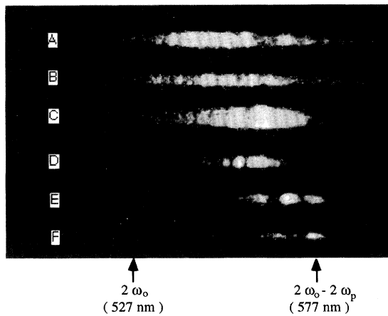
FIG. 1. Variation of second harmonic at 45° backscattered direction with respect to incident laser intensity: (a) 2.0 \times 10^{18} , (b) 1.5 \times 10^{18} , (c) 1.0 \times 10^{18} , (d) 6 \times 10^{17} , (e) 5 \times 10^{17} , and (f) 3 \times 10^{17} W/cm 2 .
